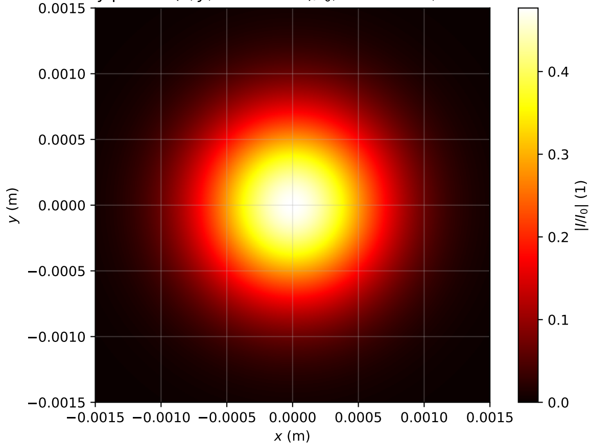
Intensity profile I(x, y, z = 2.468m)/I_0 , P_{in}=0.2P_{cr} , artificial time
